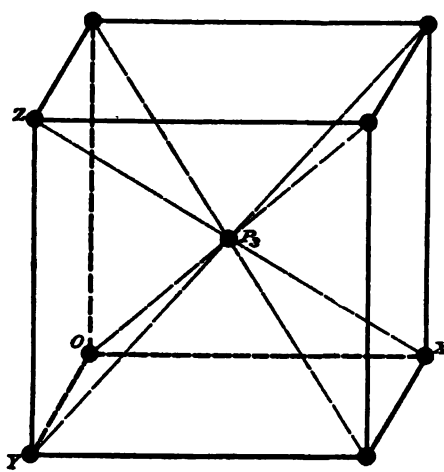
FIG. 32. A rectangular parallelepiped. If YZ \neq YO \neq OX it corresponds to \Gamma_0''' , if YZ \neq YO = OX to \Gamma_1'(b) , or if YZ = YO = OX to \Gamma_1'' .
